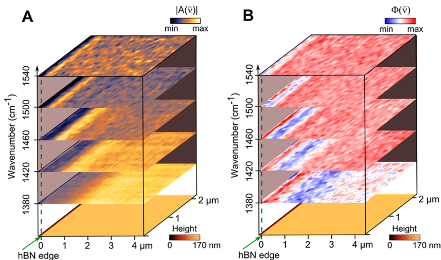
Figure 2. Sequence of real-space SINS images of near-field (A) amplitude |A(\bar{\nu})| and (B) phase \Phi(\bar{\nu}) near an edge of a 160 nm thick hBN flake acquired simultaneously. The bottom image in both (A) and (B) is the topography of the sample, showing the sample edge on the left side of the image stack at x = 0 (indicated by the dotted green line). The color maps for the amplitude and phase images have been individually normalized to the maximum and minimum amplitude and phase value of each image for better visibility. Interference between the forward-propagating and back-reflected polariton waves modulates the near-field amplitude and phase as a function of the distance from the hBN edge. Different interference patterns are due to different polariton wavelengths.
