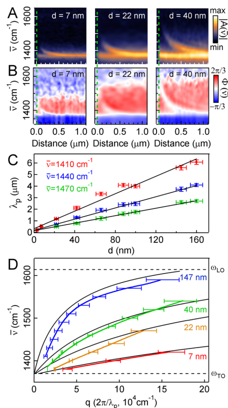
Figure 6. PhP dispersion and evolution of the in-plane phonon polariton wavelength with sample thickness. Spatospectral maps of (A) SINS amplitude |A(\bar{\nu})| and (B) phase \Phi(\bar{\nu}) for samples with thicknesses of 7, 22, and 40 nm. (C) Evolution of the in-plane phonon polariton wavelength, \lambda_p , with sample thickness, d , at three representative excitation frequencies: 1410, 1440, and 1470 \text{cm}^{-1} . For thin hBN flakes, \lambda_p is proportional to sample thickness. (D) Experimental (colored curves) and theoretical (black curves) dispersion relations of in-plane PhPs on hBN flakes with different thicknesses. The horizontal dashed lines are the longitudinal ( \omega_{\text{LO}} = 1614 \text{ cm}^{-1} ) and transverse ( \omega_{\text{TO}} = 1370 \text{ cm}^{-1} ) optical phonon frequencies of hBN.
