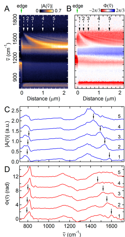
Figure 3. Spatio-spectral SINS line scan of hBN phonon polaritons with spectral cuts. Simultaneously acquired (A) near-field amplitude |A(\bar{\nu})| and (B) phase \Phi(\bar{\nu}) linescan obtained perpendicular to the edge of a 147 nm thick hBN flake. The green arrow at x = 0 marks the edge of the hBN crystal. Signals around 1370 and 780 \text{cm}^{-1} correspond to the in-plane and out-of-plane phonon mode in hBN, respectively, and the signal around 1130 \text{cm}^{-1} is related to the \text{SiO}_2 phonon mode of the substrate. Strong PhP features only appear around the in-plane phonon mode (1370 \text{cm}^{-1} ). Near-field (C) amplitude and (D) phase spectra at five representative positions, marked in (A) and (B).
