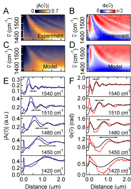
Figure 4. Cavity model analysis of experimental spatial and spectral profiles. Experimental (A) SINS amplitude |A(\bar{\nu})| and (B) phase \Phi(\bar{\nu}) spatio-spectral linescan in the region of the hBN in-plane phonon mode of the 147 nm thick hBN flake. Note the different color scales from Figure 3 with absolute phase values. Simulated SINS (C) amplitude and (D) phase spatio-spectral linescan of the same hBN flake in (A) and (B) using the cavity model discussed in the text. (E) Experimental (blue) and simulated SINS amplitude (black) distance profiles extracted from (A) and (C), respectively. (F) Experimental (red) and simulated SINS phase (black) distance profiles extracted from (B) and (D), respectively.
