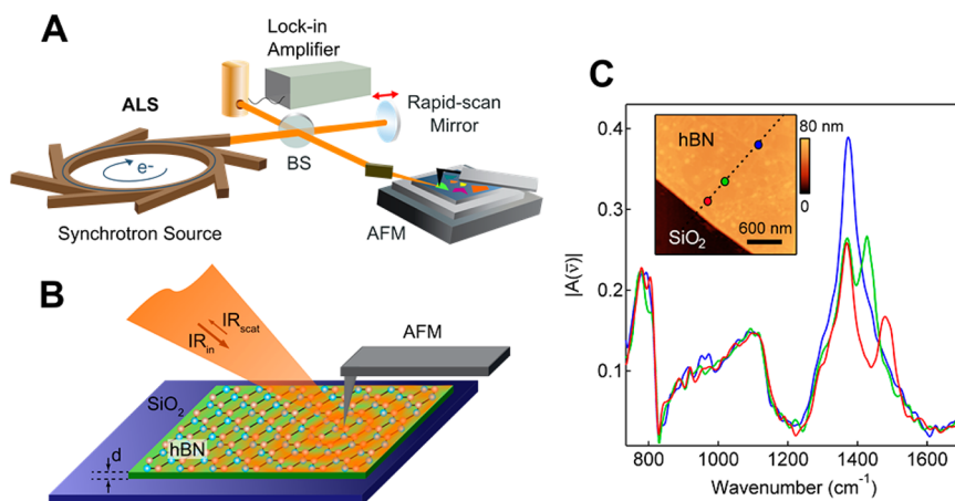
Figure 1. (A) Schematic of synchrotron infrared nanospectroscopy (SINS) using coherent broadband synchrotron infrared radiation provided by the Advanced Light Source (ALS) as the synchrotron source, a KBr beamsplitter (BS), and an atomic force microscope (AFM). (B) The synchrotron IR light illuminates the conductive AFM tip, which launches polariton waves that propagate radially outward from the tip along the hBN surface and are reflected off the edges, forming standing waves with the tip. (C) Representative amplitude |A(\bar{\nu})| spectra taken from three different positions (marked with colored dots) of a 75 nm thick hBN flake, shown in the inset. A peak appears on the high-frequency side of the main in-plane phonon peak near 1370\text{ cm}^{-1} in the spectra taken near the hBN edge, due to the interference of the forward-moving and backward-moving polariton wave reflected by the hBN edge.
