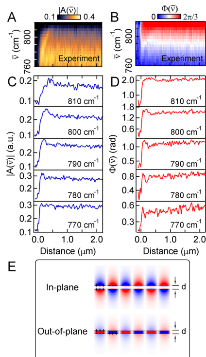
Figure 5. Experimental (A) SINS amplitude |A(\bar{\nu})| and (B) phase \Phi(\bar{\nu}) spatio-spectral linescan in the region of the hBN out-of-plane phonon mode of the 147 nm thick hBN flake. Experimental amplitude (C) and phase (D) distance profiles extracted from (A) and (B), respectively. (E) Color map of the electrical field along the c -axis for the fundamental in-plane (top) and out-of-plane (bottom) phonon polariton modes.
